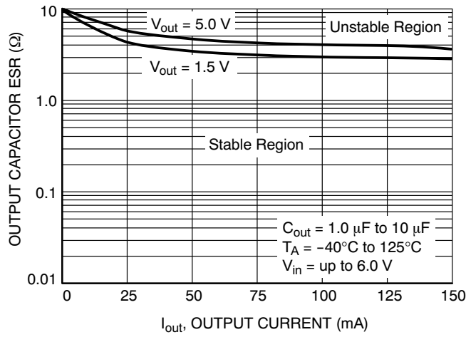
Figure 23. Output Stability with Output Capacitor ESR over Output Current
